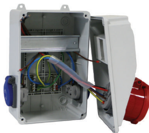
IP44 Cable Mounted Combination Box
